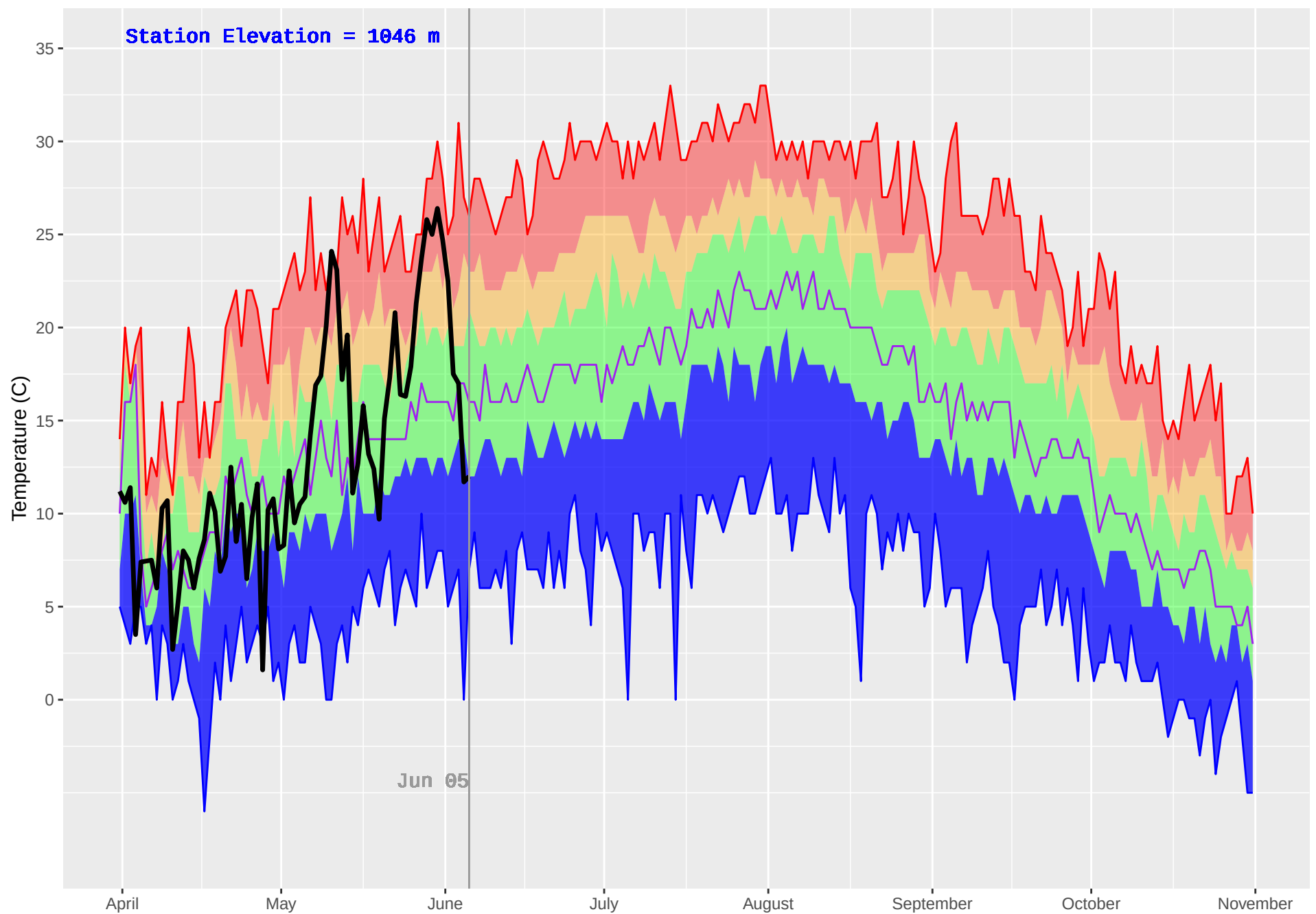
LIKELY RS (255) : Historical (1970–2018) and Current (2019) Daily Temperature
