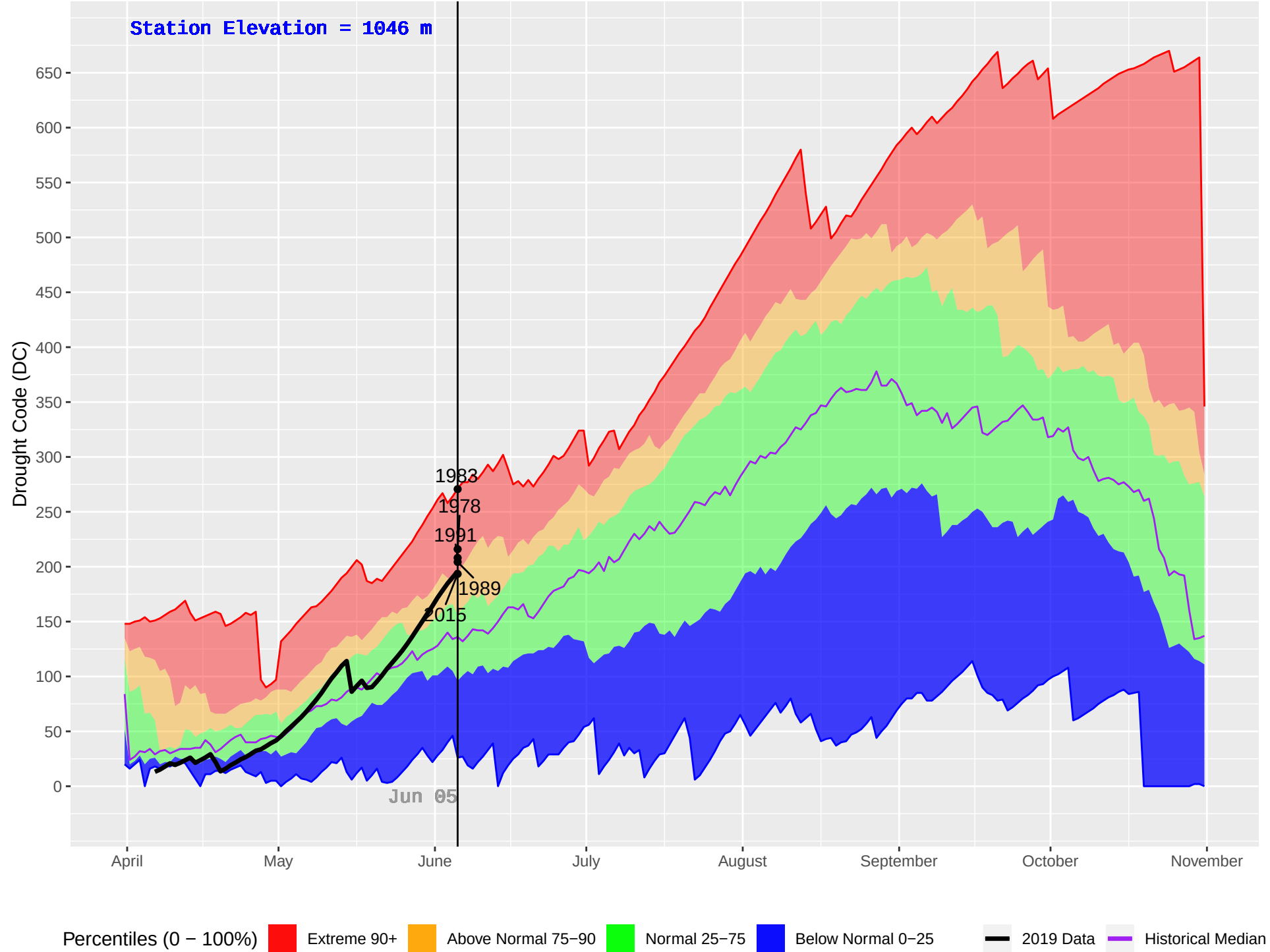
LIKELY RS (255) : Historical (1970–2018) and Current (2019) Daily Drought Code (DC)
