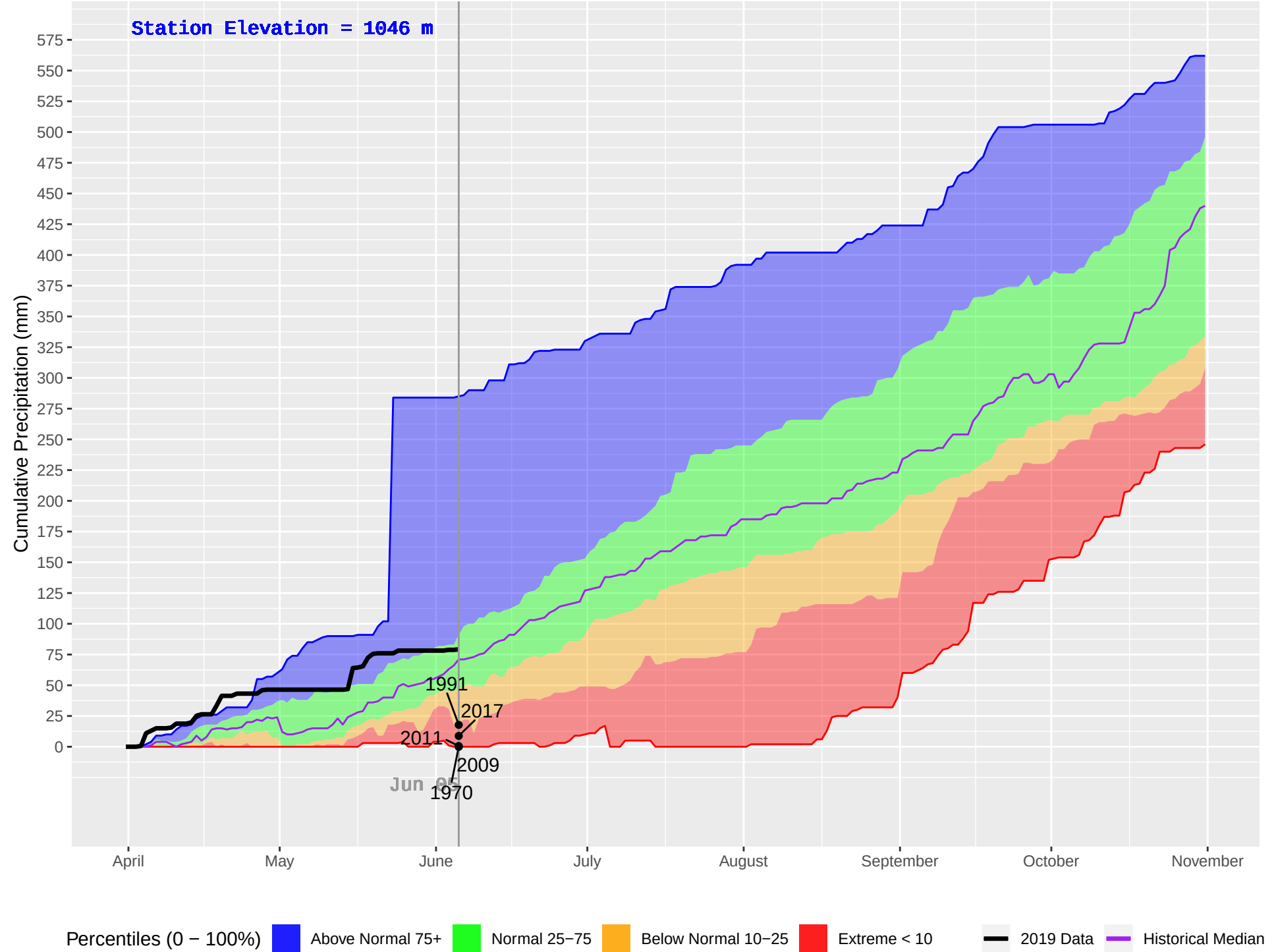
LIKELY RS (255) : Historical (1970–2018), Current (2019) Daily Cumulative Precipitation
