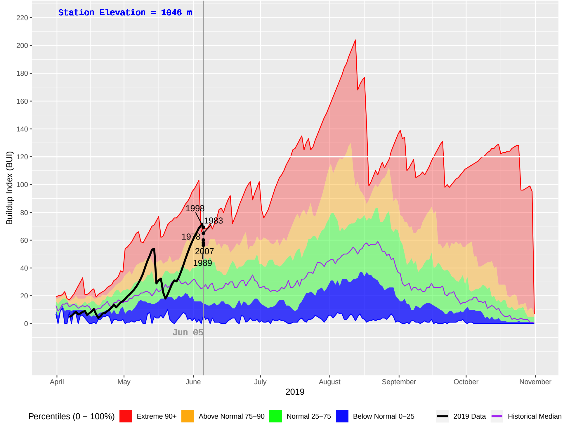
LIKELY RS (255) : Historical (1970–2018), Current (2019) Daily Buildup Index (BUI)
