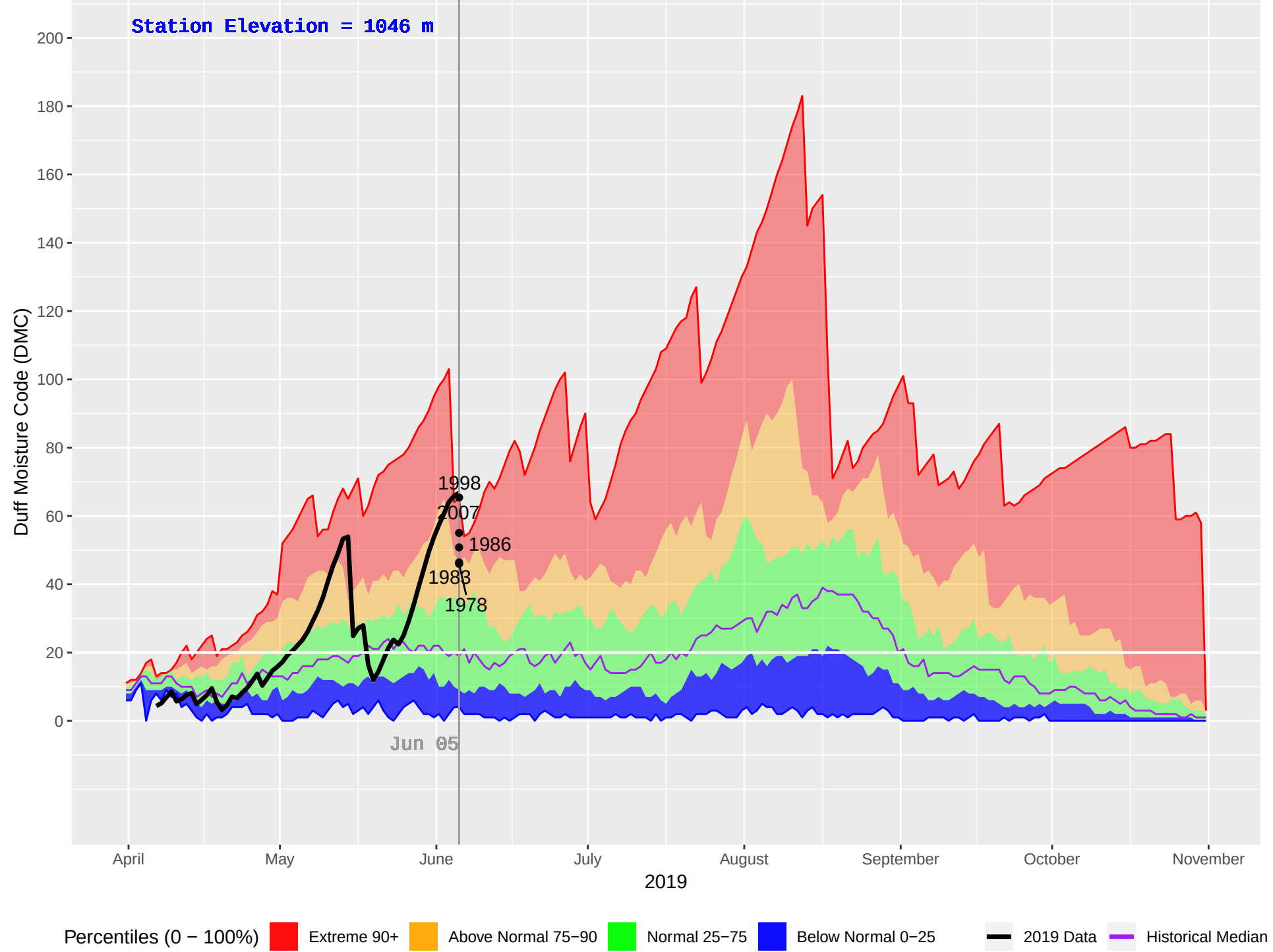
LIKELY RS (255) : Historical (1970–2018), Current (2019) Daily Duff Moisture Code (DMC)
