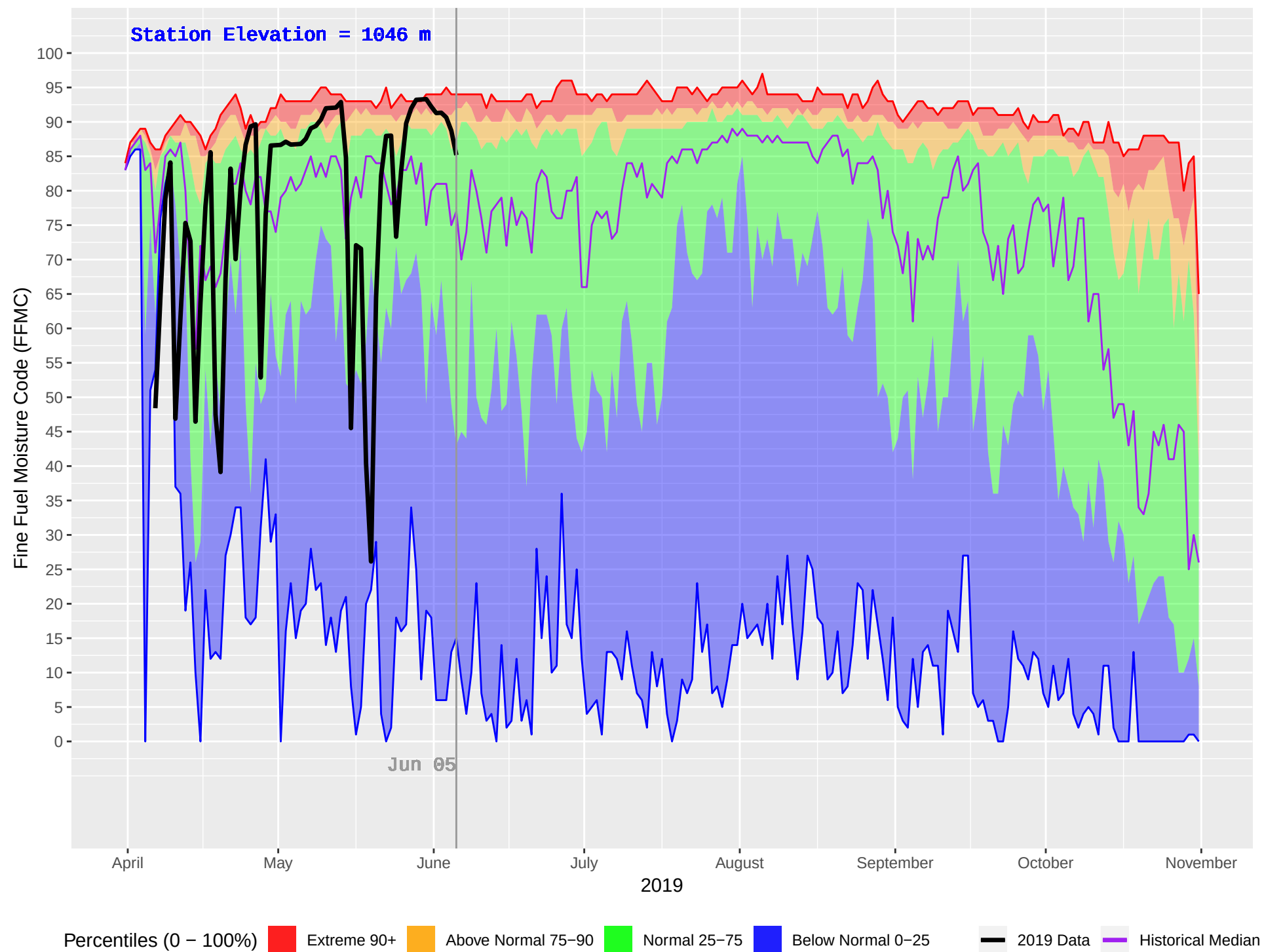
LIKELY RS (255) : Historical (1970–2018) and Current (2019) Daily Fine Fuel Moisture Code (FFMC)
