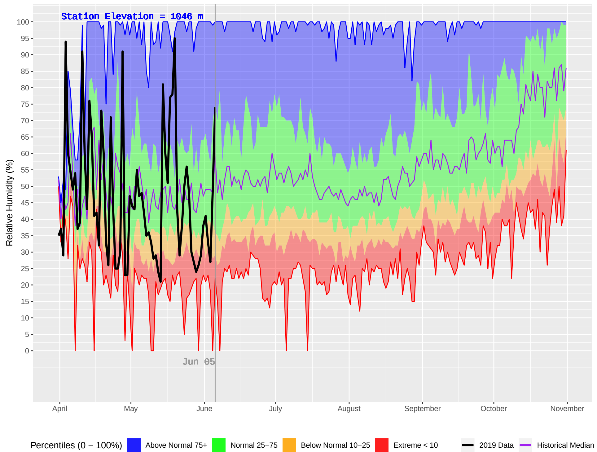
LIKELY RS (255) : Historical (1970–2018) and Current (2019) Daily Relative Humidity
